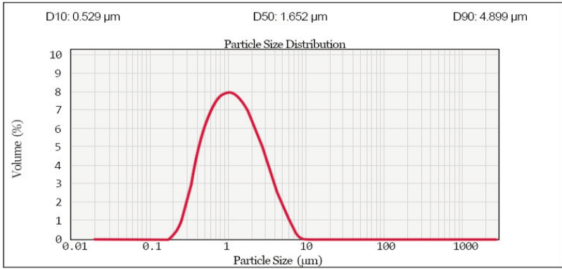
Ceroxid HD W1520 PSD laser particle size distribution analyzer
